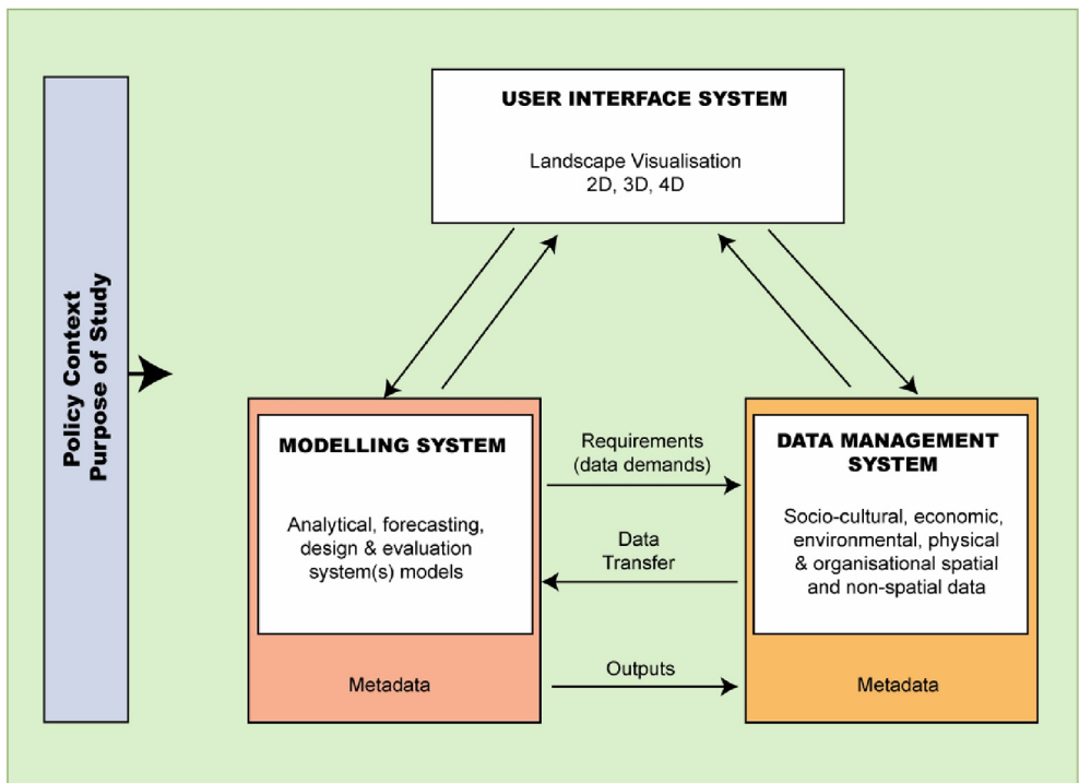
Figure 1 Generic Spatial Decision Support System
